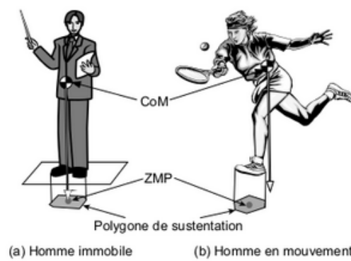
Figure 3.3 – CoM, ZMP et polygone de sustentation.
